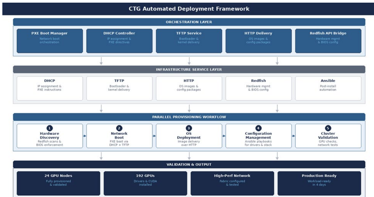
Figure 1: CTG Automated Deployment Framework
